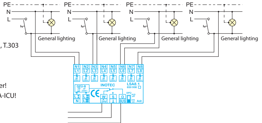
BUS- connection
